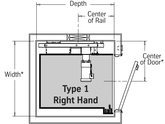
Type 1 - Right Hand Car with Pocket Gate Gate Stack - Opposite Rail
